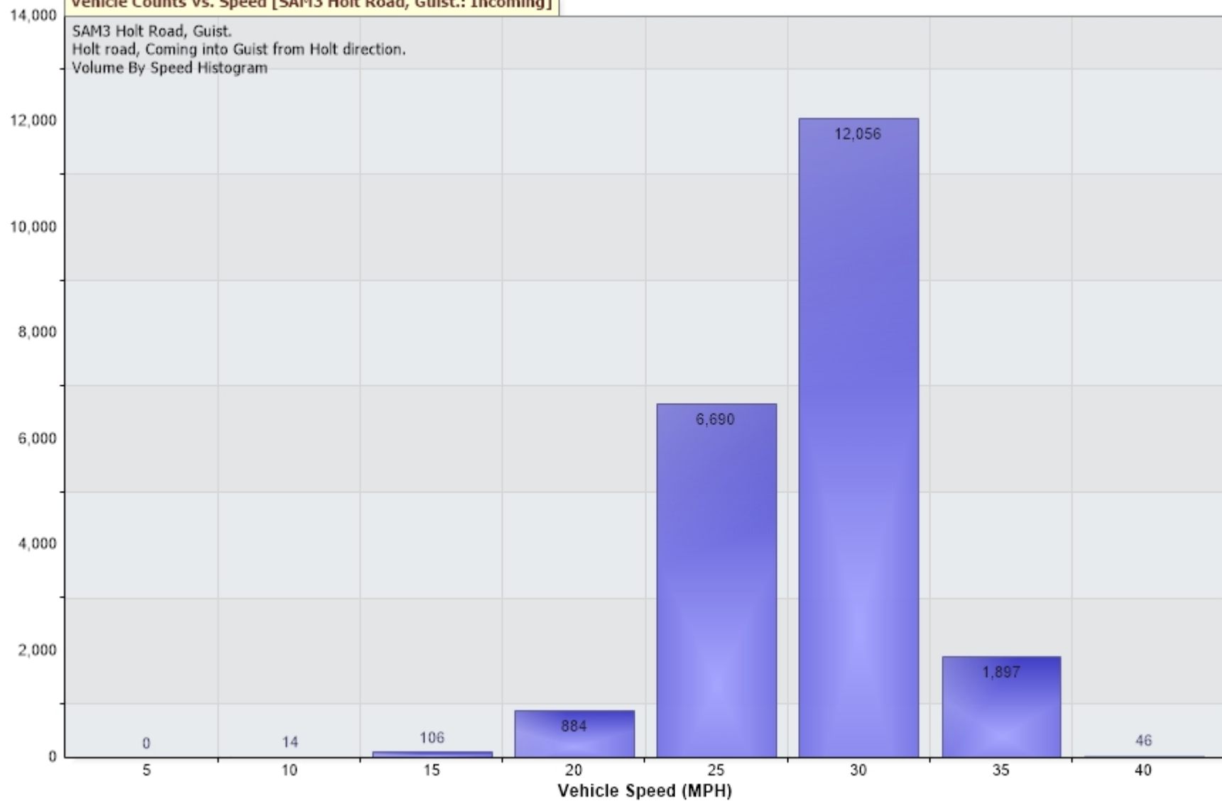
Vehicle Counts Vs. Speed [SAM3 Holt Road, Guist.: Incoming]
